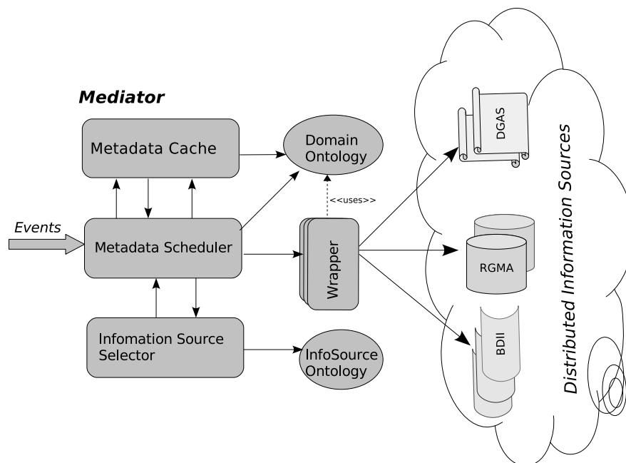
Figure 1: Overview of the Active Ontology architecture [8]
