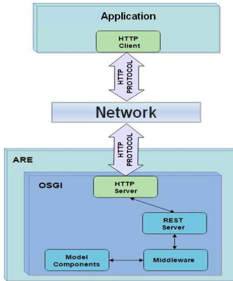
Figure 3. The REST-enabled AsTeRICS architecture.
