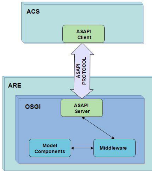
Figure 2. The original AsTeRICS architecture.
